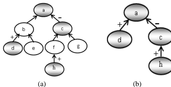
Figure 6 The tree rule extraction search
