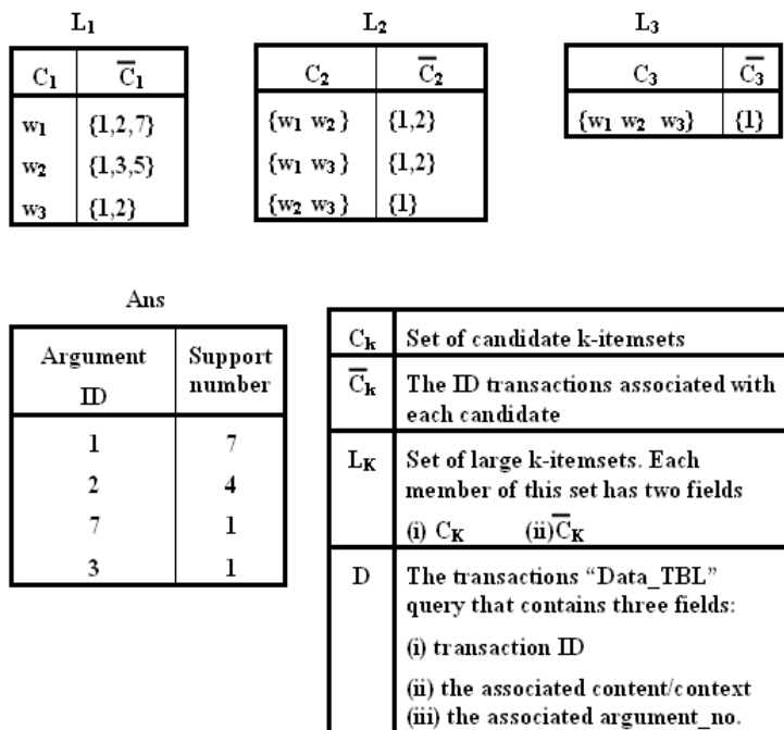
Figure 5 The adapted AprioriTid mechanism
