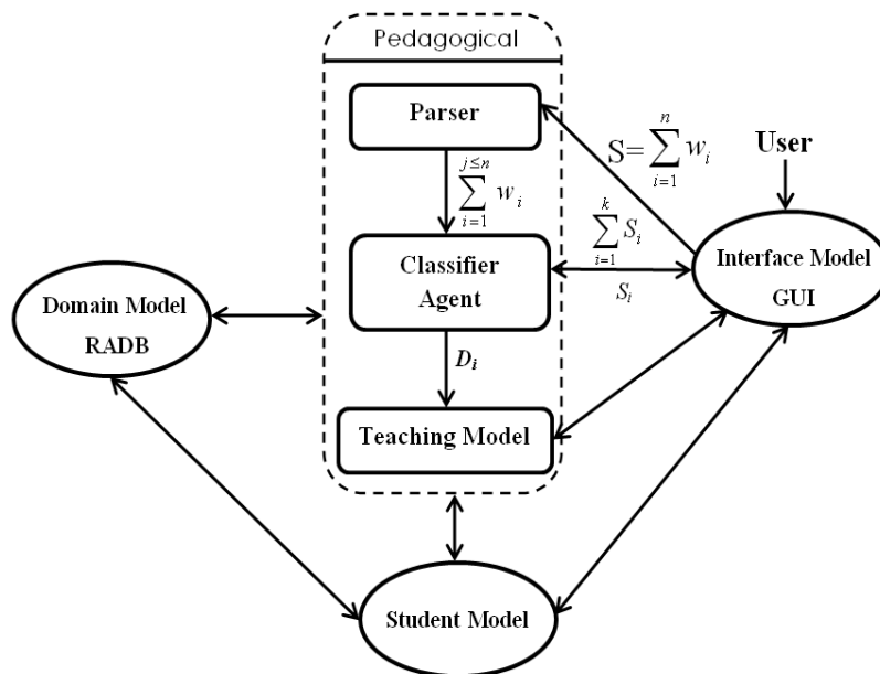
Figure 1 ALES architecture
